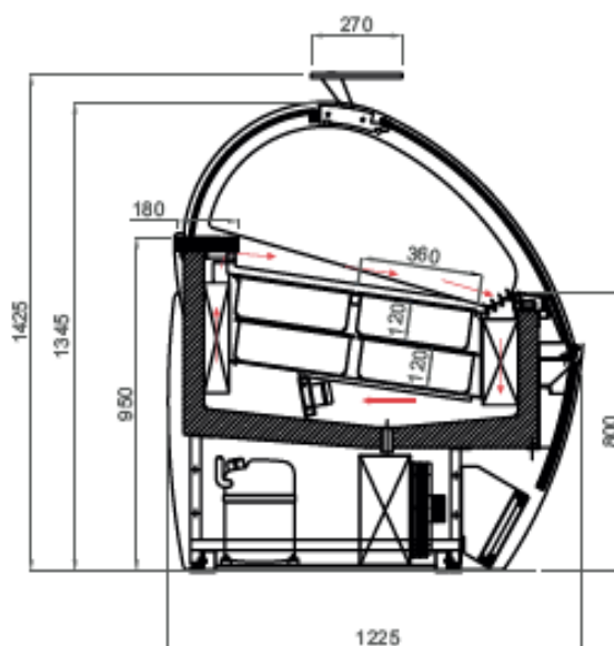
Double ventilation
