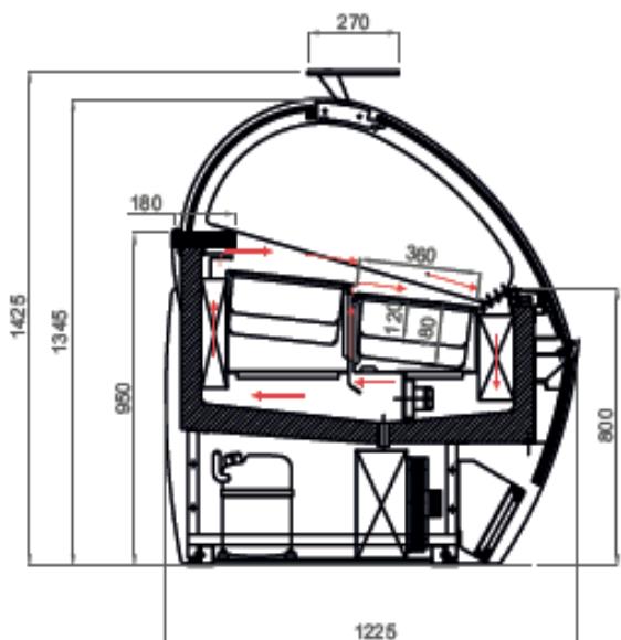
Simple ventilation
